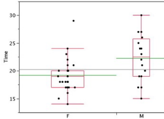
Figure 1.14: Box plots with the individual scores jittered.
