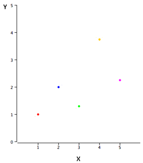
Figure 3.8: A scatter plot of the example data.
