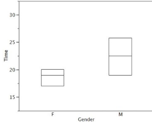
Figure 1.9: The first step in creating box plots.
